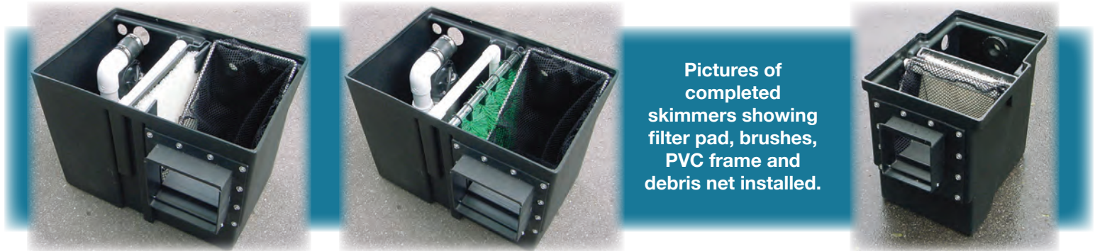
Skimmer w/Filter Pad • Part #PS1V Skimmer w/Filter Brushes • Part #PS1FB
