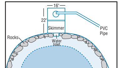
Skimmer location without extension tube.
