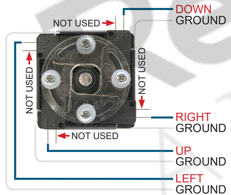
JOYSTICK WIRING
