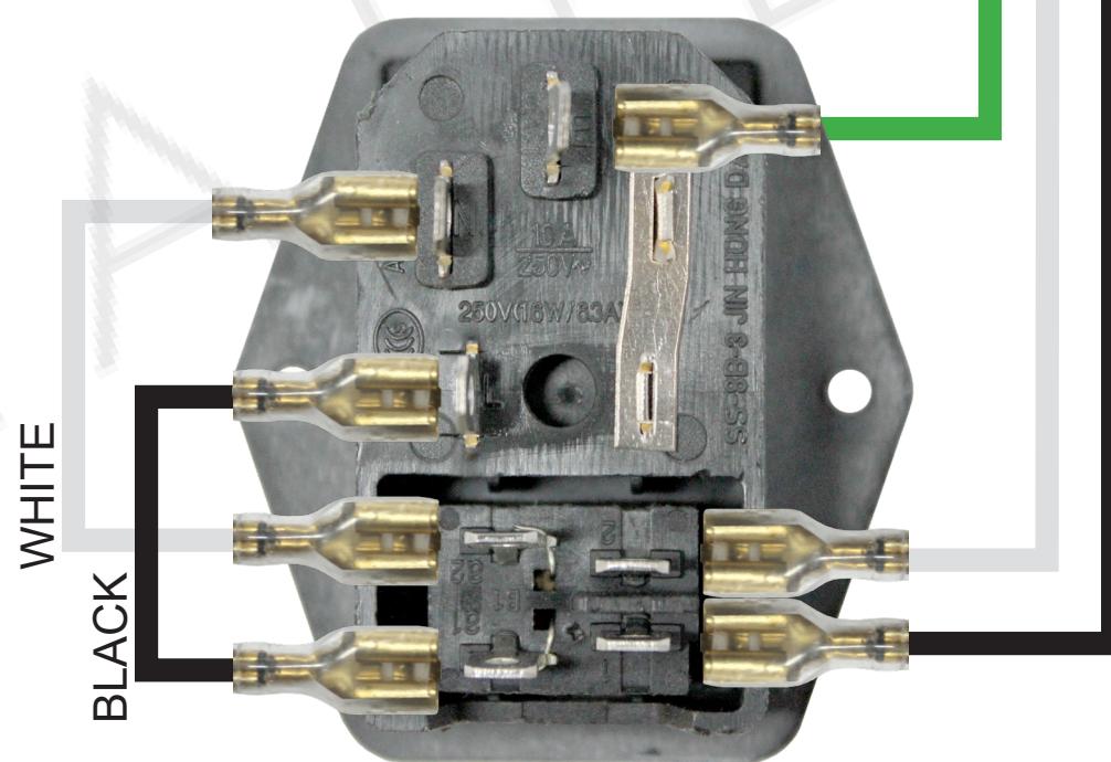
Back View
