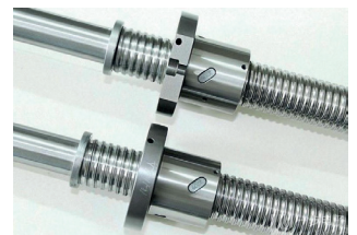
Dual Ballscrew
