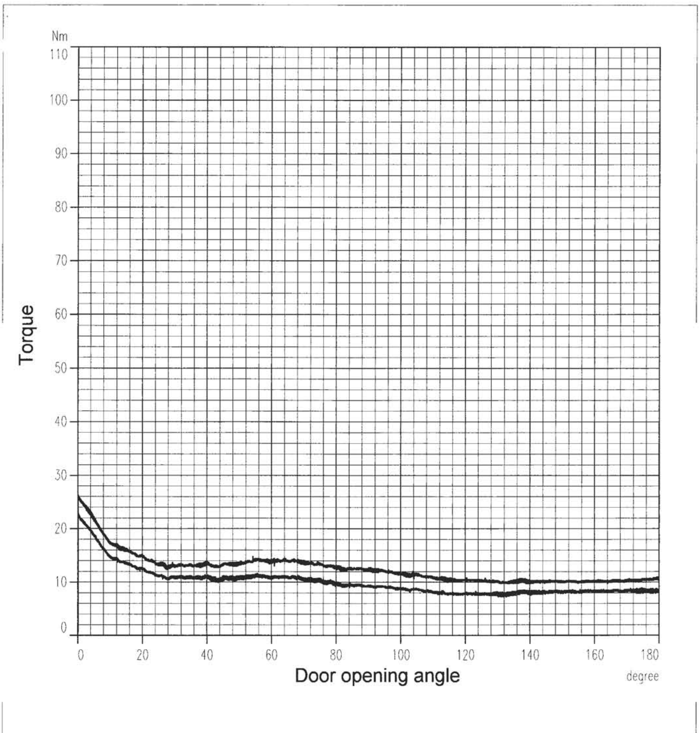
Torque curve
