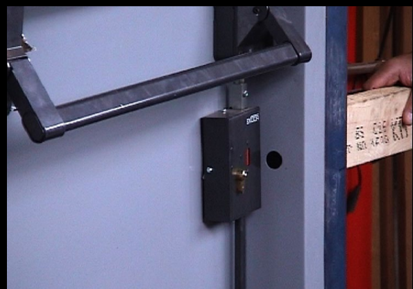
Inside view shows the door is held closed.
