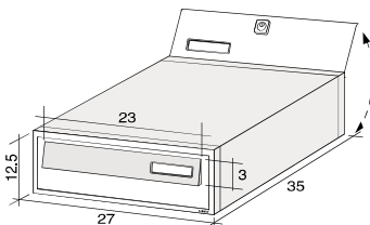
Modular 270/2 completa - Modular 270/2 complete box
