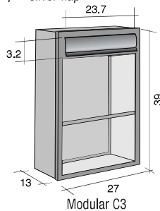
Modular C3 CAR con cornice di plastica argento ed el. mob. color argento with silver plastic frame and silver flap
