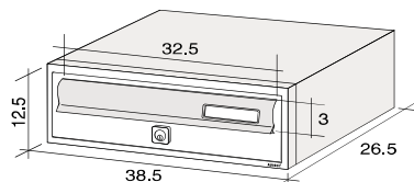
Modular 1 completa Modular 1 complete box
