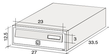
Modular 270 completa - Modular 270 complete box
