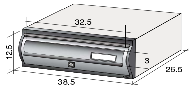
CURVE 1 completa - CURVE 1 complete box
