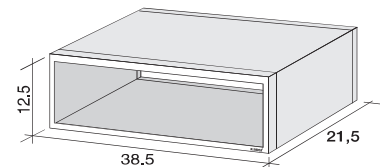
Modular 2002
