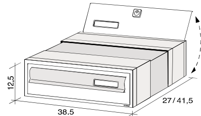
Modular 2 T completa - Modular 2 T complete box
