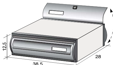
CURVE 2 completa - CURVE 2 complete box
