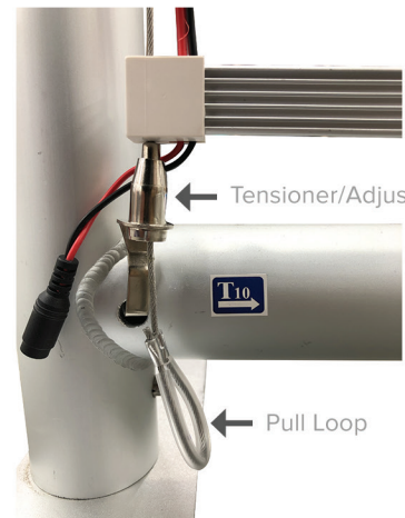
LED Light Installation Bottom Connection Insert hooks into holes along bottom tube Bottom of lights have a pull loop and adjuster to add tension to lights
