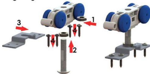
Hanger for timber doors (pair)
