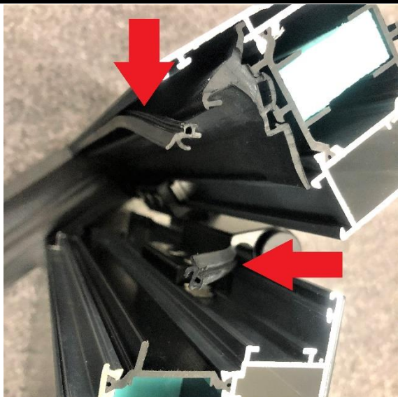
ThruSafe (TLS 90) Frame & Sash Flipper Gasket 1/6
