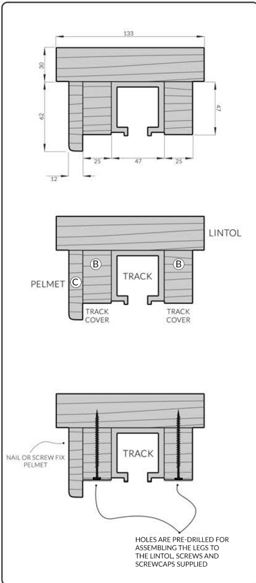
SECTION H - H
