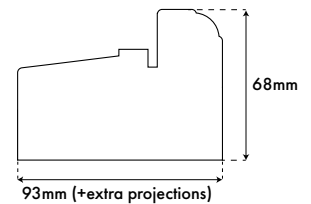
FRAME CILL (OPENS OUT)
