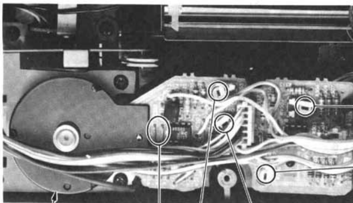
RV503 RV504 offset adjustment output to motor coil
