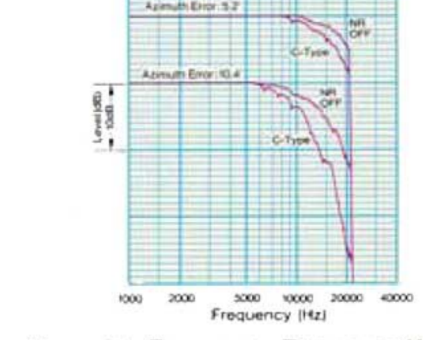
Figure 7 Frequency Response With 5.2' & 10.4' Azimuth Error With & Without Dolby-C NR Deck: CR-7/Level: -20dB/PB Eq: 70µs/Tape: ZX (Metal)
