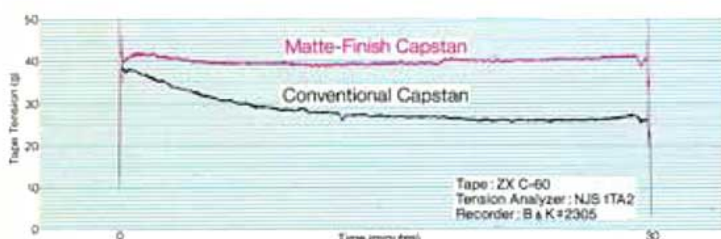
Figure 11 Tape Tension Comparison
