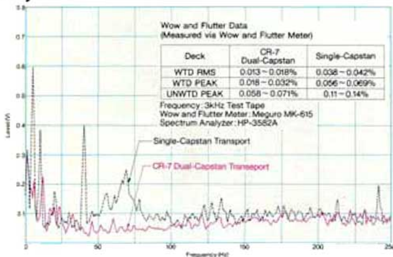
Figure 10 CR-7 Flutter Analysis
