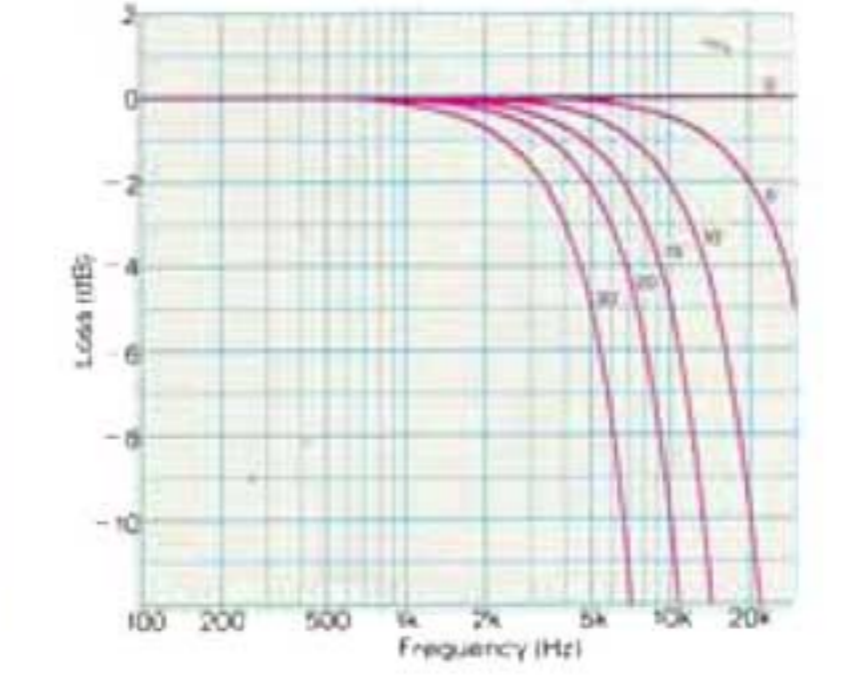
Figure 6 Azimuth Misalignment Loss vs Frequency
