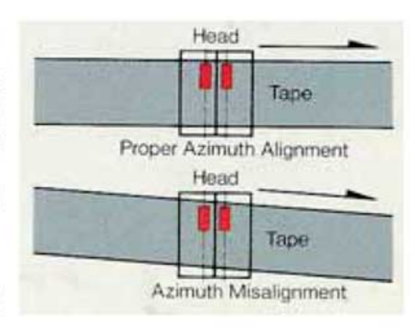
Figure 5 Azimuth Misalignment
