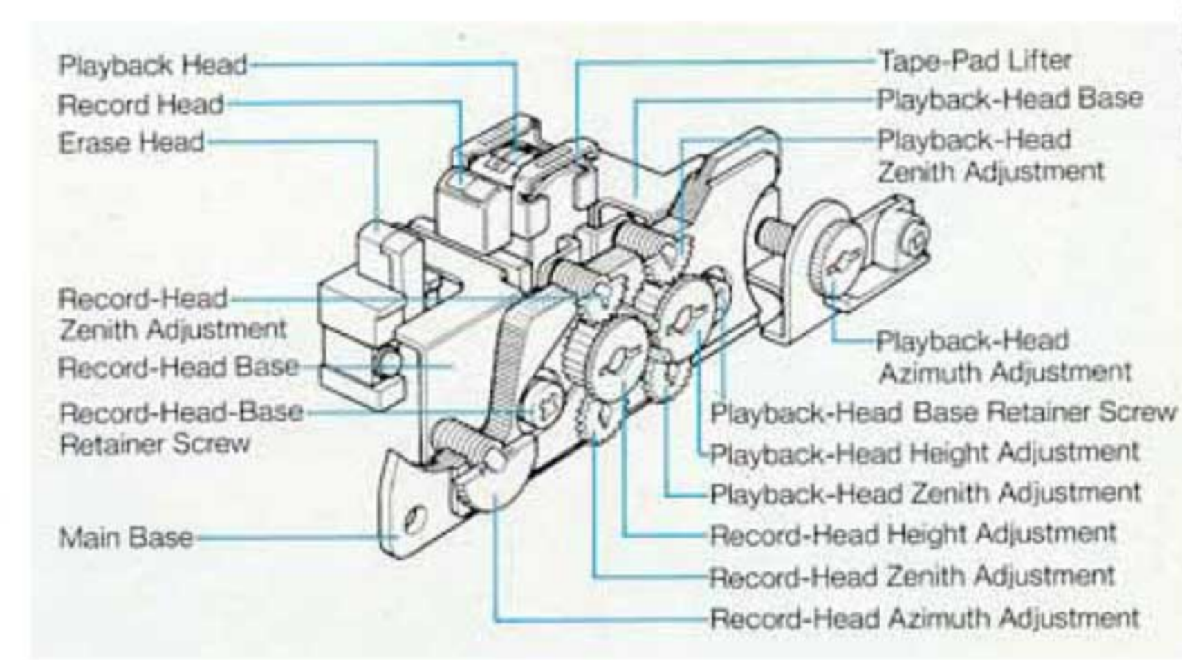
Figure 8 Discrete Three-Head Mounting Arrangement
