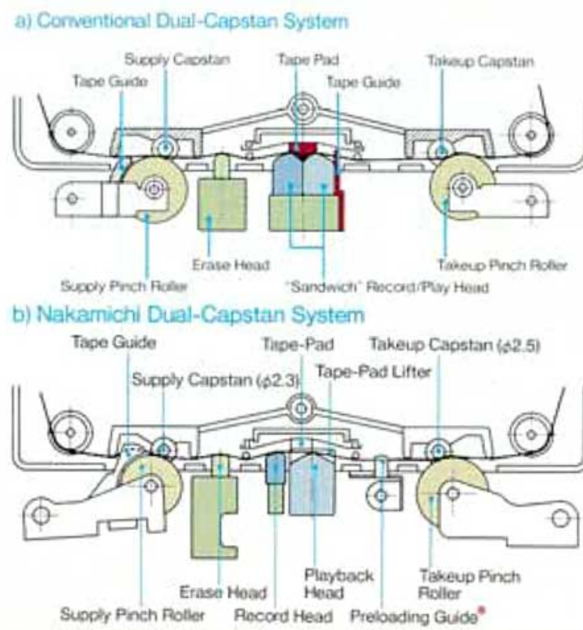
Figure 12 Tape Path In A Dual-Capstan System
