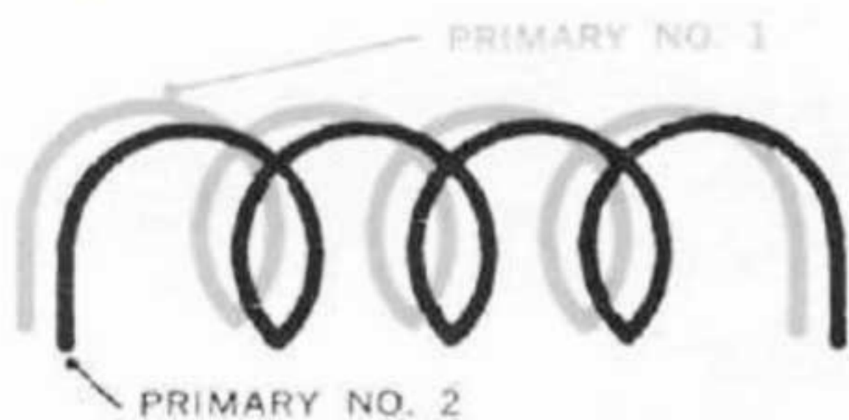
Fig. 1 — Representation of bifilar winding.
