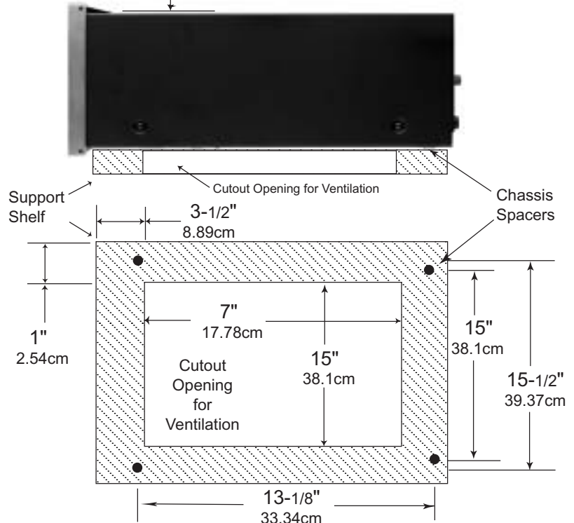
MA6500 Bottom View in Custom Cabinet
