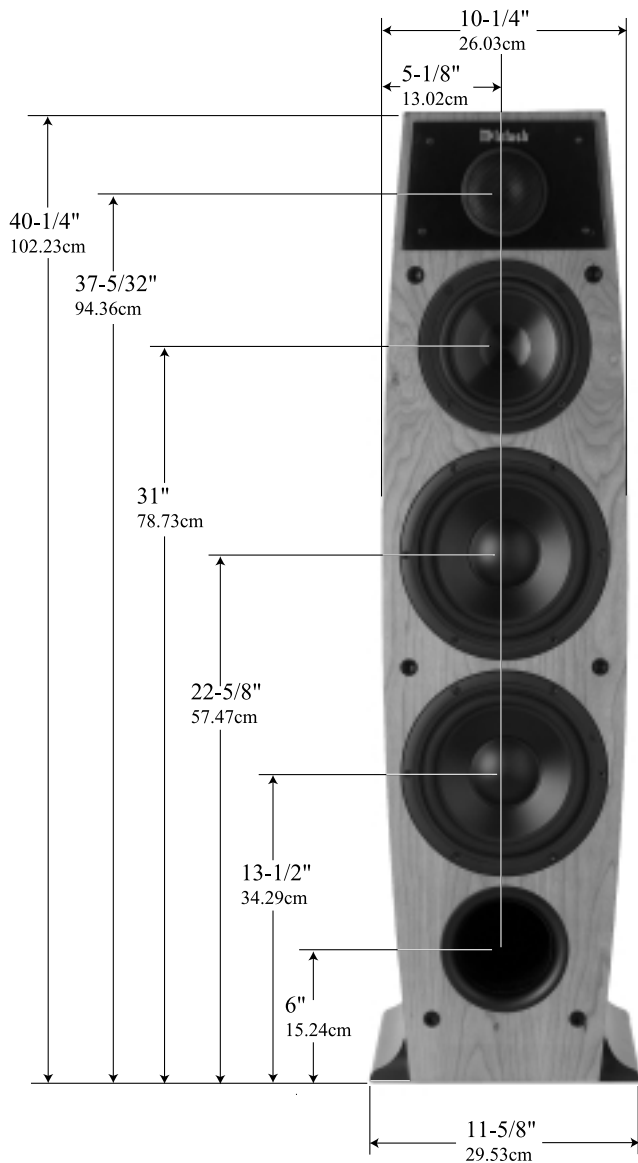
Front View of LS340 with Grille Removed
