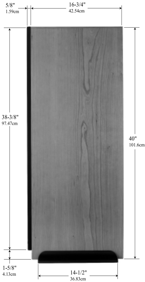
Side View of LS340 with Grille
