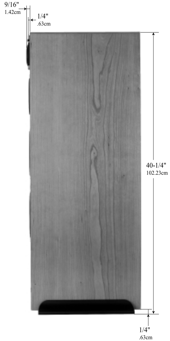
Side View of LS340 with Grille Removed
