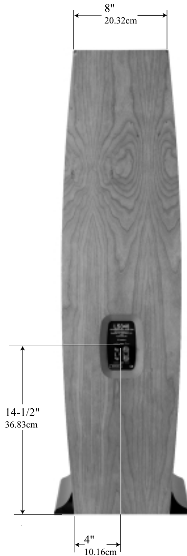
Rear View of LS340
