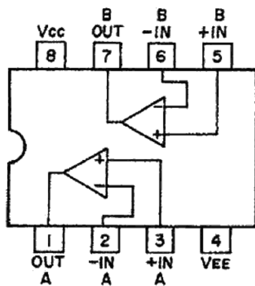
NJM4558D
