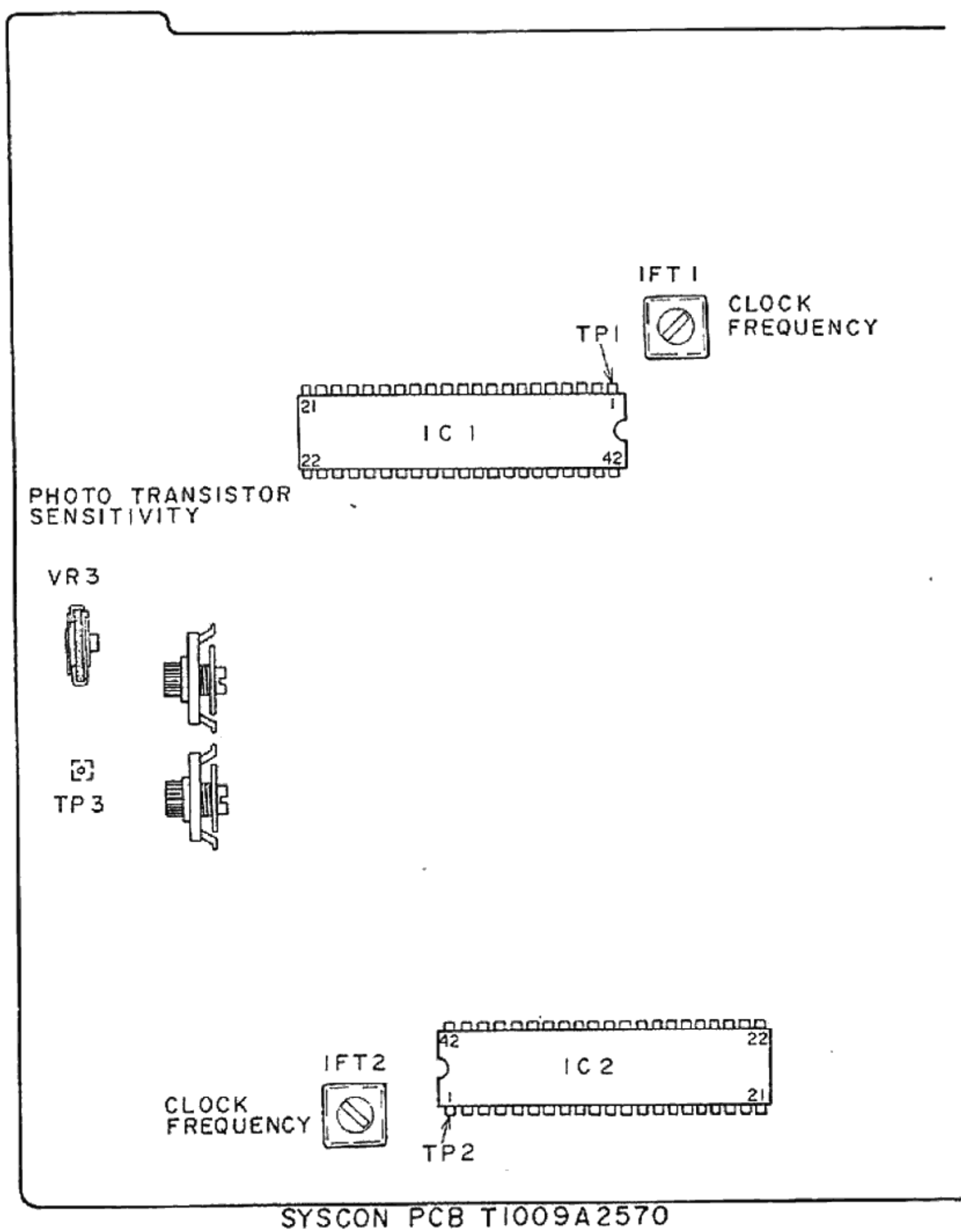
Fig. 44 Syscon P.C Board T1009A2570
