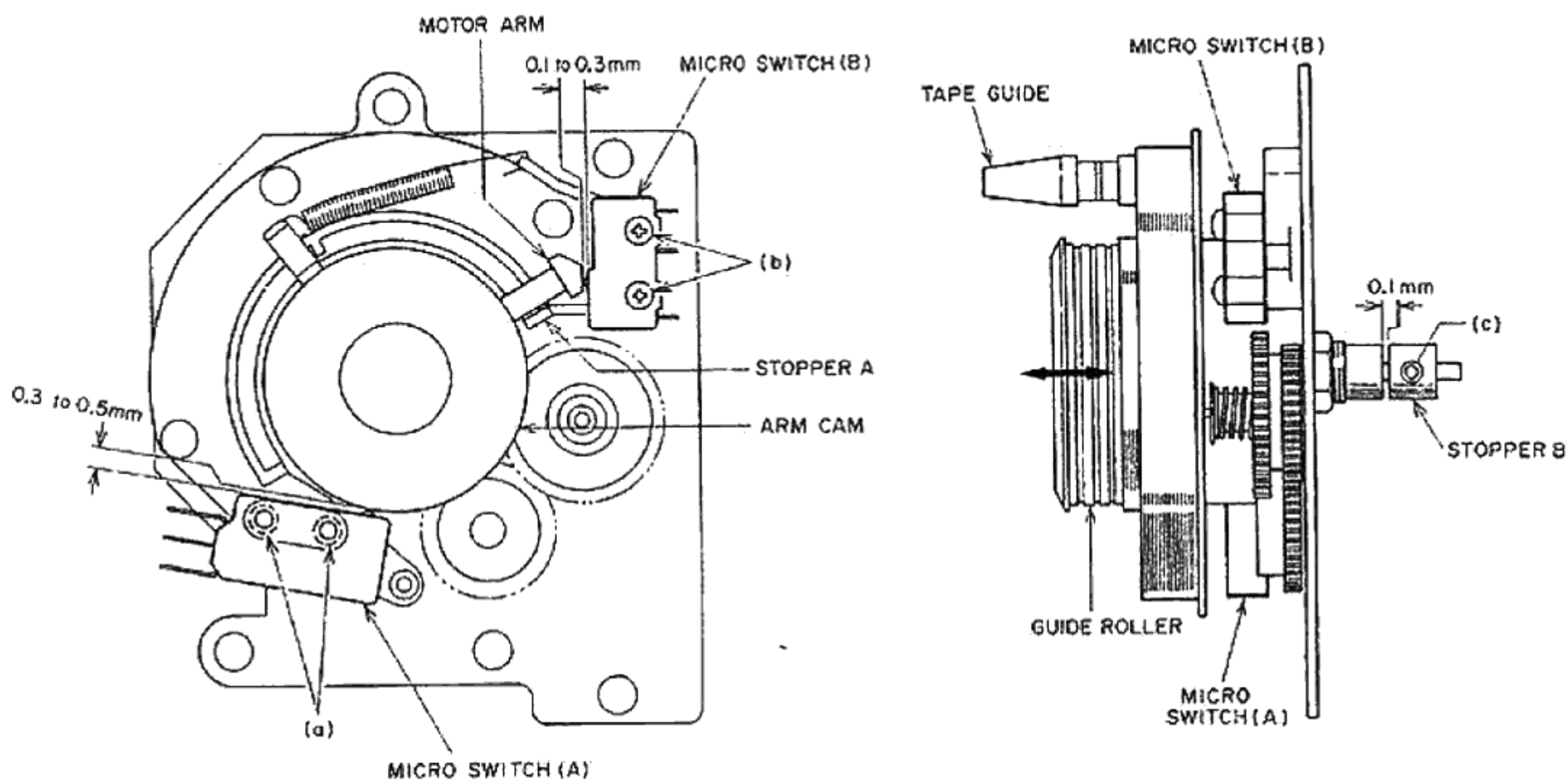
Fig. 33 Roller Block
