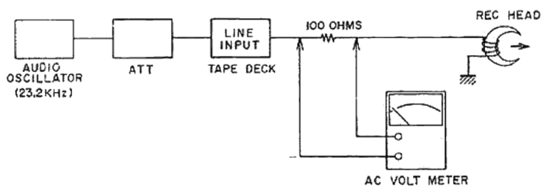
Fig. 47 Rec Peaking Adjustment Instrument Connection
