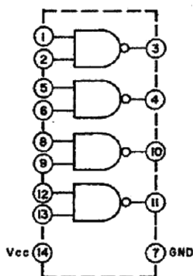
MC14011BCP
