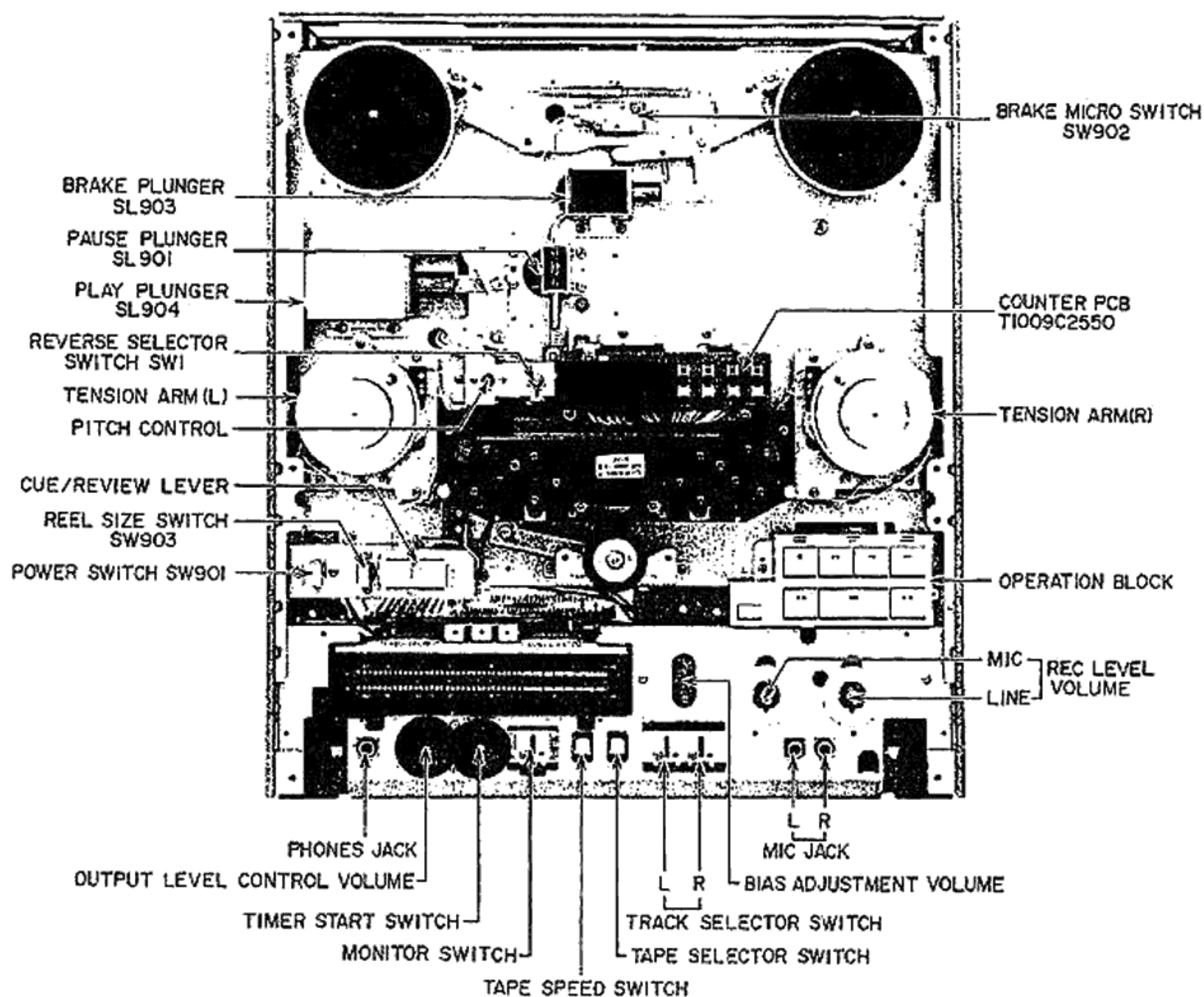
Fig. 2 Front View
