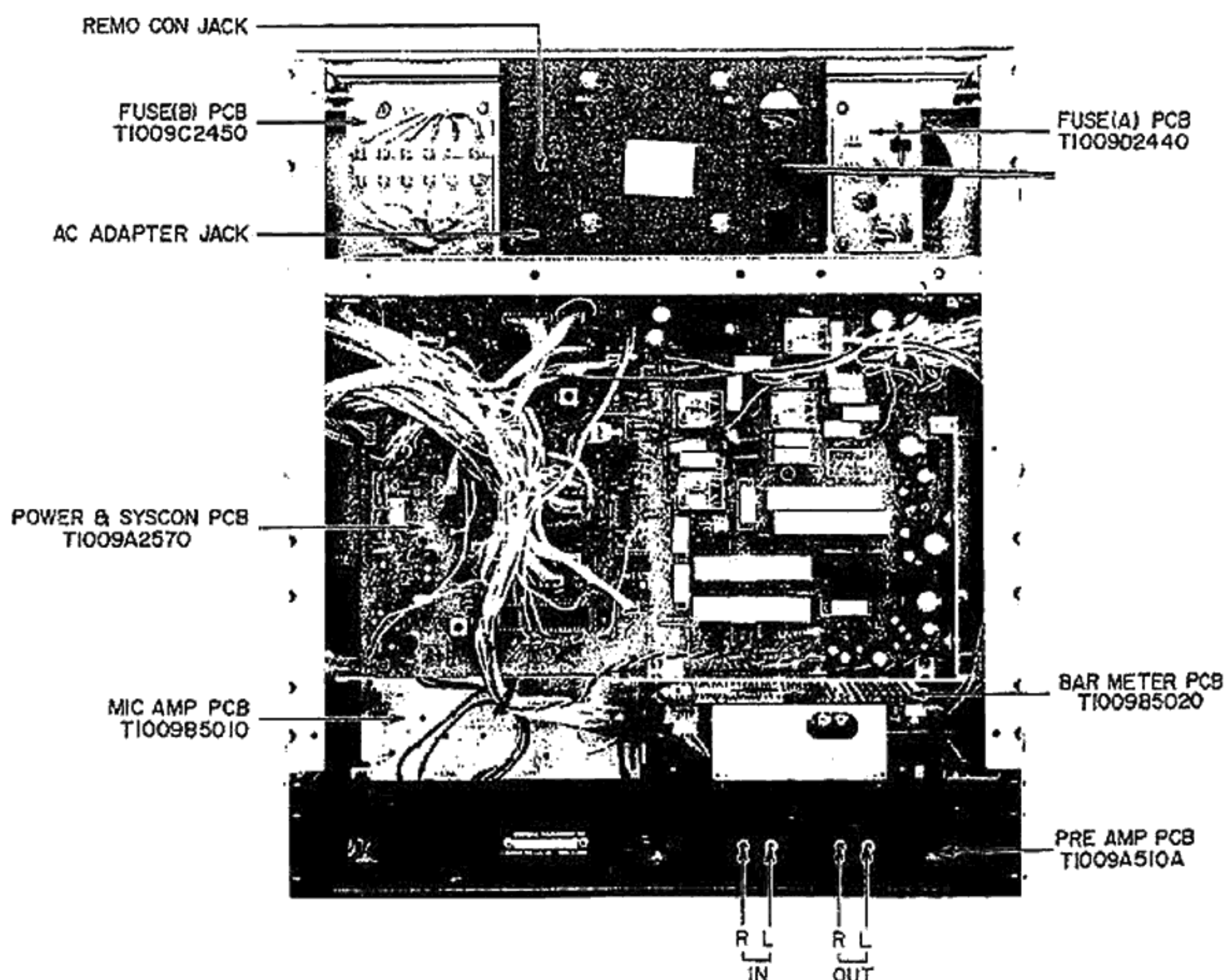
Fig. 3 Rear View
