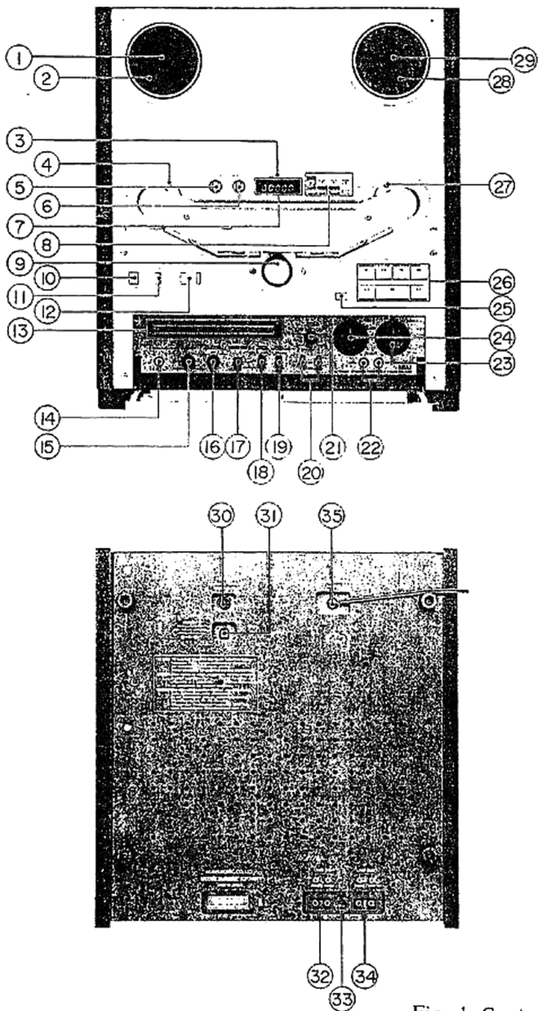
Fig. 1 Controls
