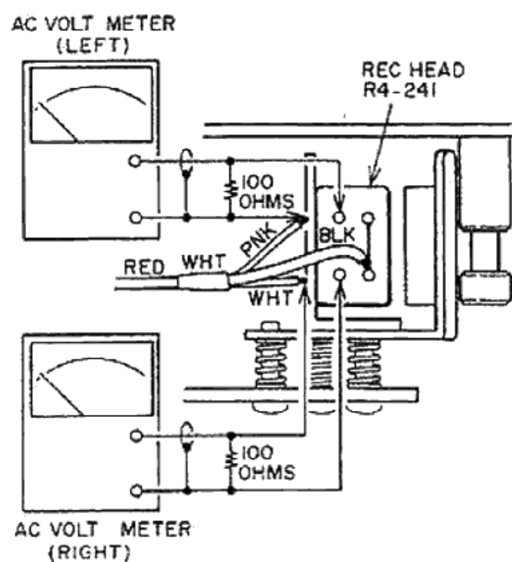
Fig. 48 Rec Peaking Adjustment
