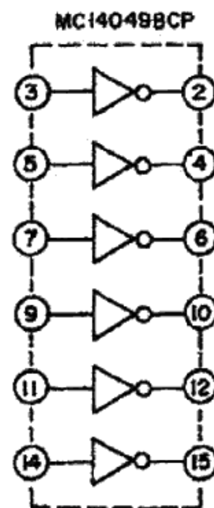
MC14049BPC
