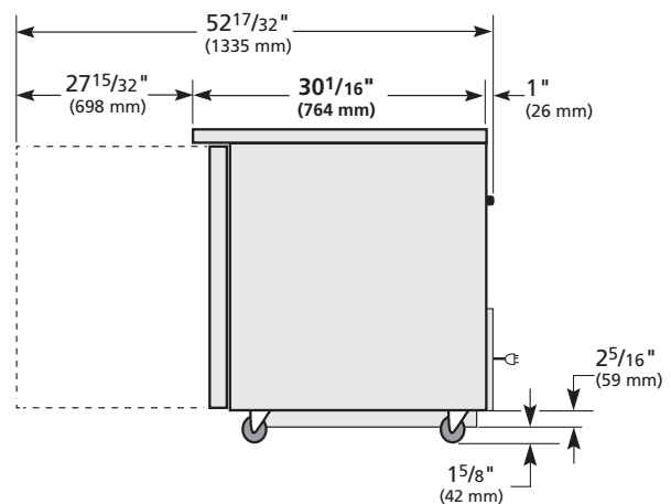
RIGHT VIEW
