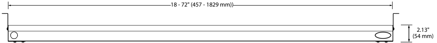
FRONT VIEW
