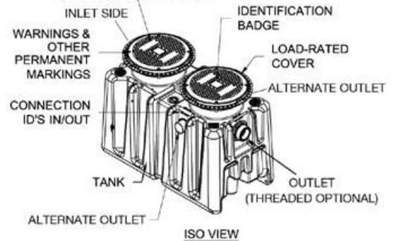
ISO VIEW
