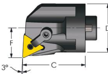
Negative Triangle (-3° Lead) Coolant Thru
