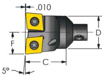
Positive 80° Diamond (-5° Lead) Turn & Bore Coolant Thru
