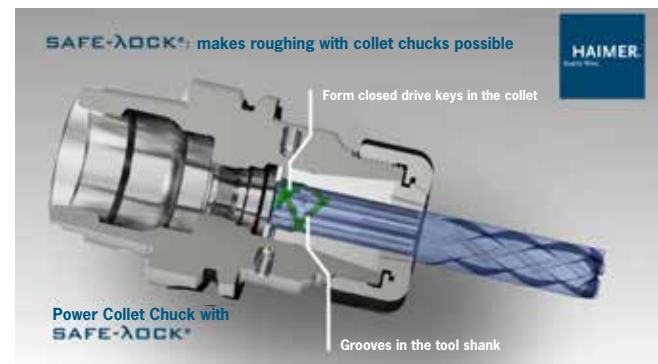
Power Collet Chuck with SAFE-LOCK®
