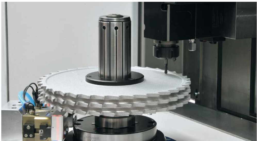
Balancing of PCD jointing cutters for laminate Balancing enables the best edge quality for the piece of furniture by vibration-free tool run. In addition the noise while machining is reduced to a minimum.
