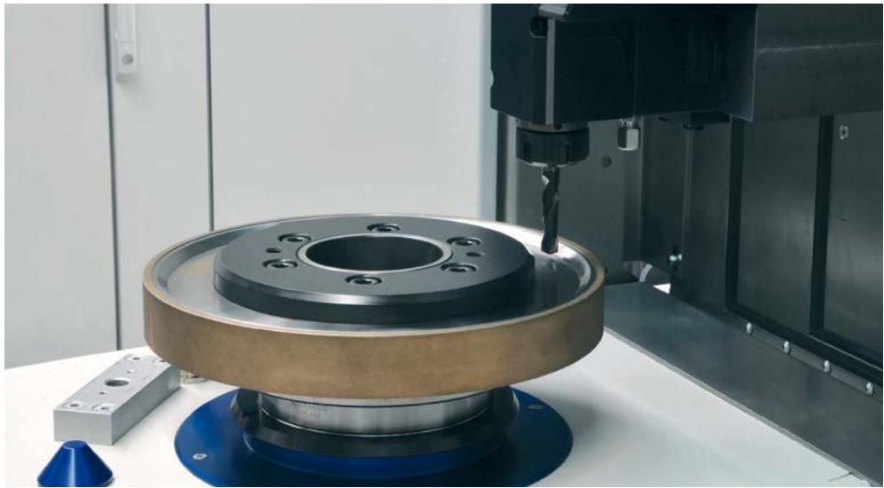
Balancing of grinding wheels by axial drilling Balanced grinding wheels reduce the surface roughness of the work piece which leads to a remarkable increase of the process performance and to a higher precision of the end product.
