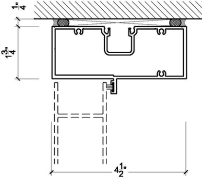
3. Top Rail Detail
