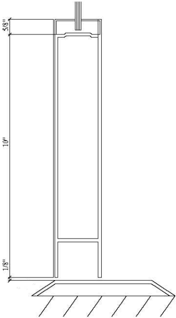
2. Bottom Rail Detail
