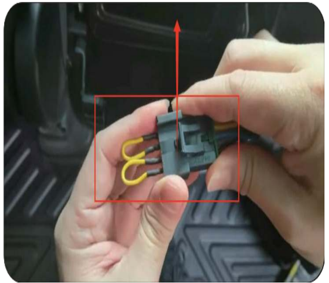
14. After plugging in the dedicated plug for the Model Y, insert it into the air vent
