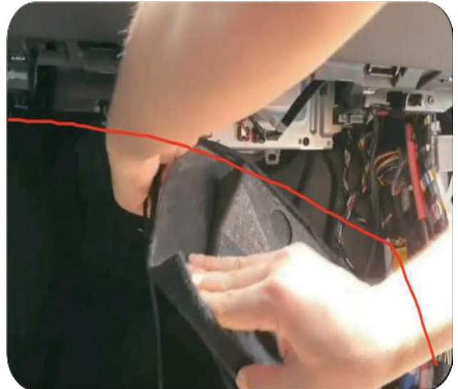
10. Route the wiring along the edge of the lower cover panel
