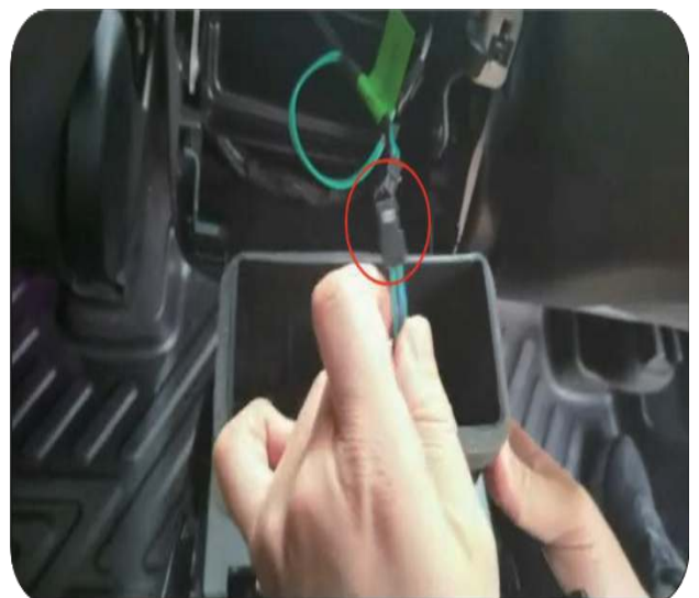
18. After connecting the power cable to the screen, restore the vehicle to its original state
