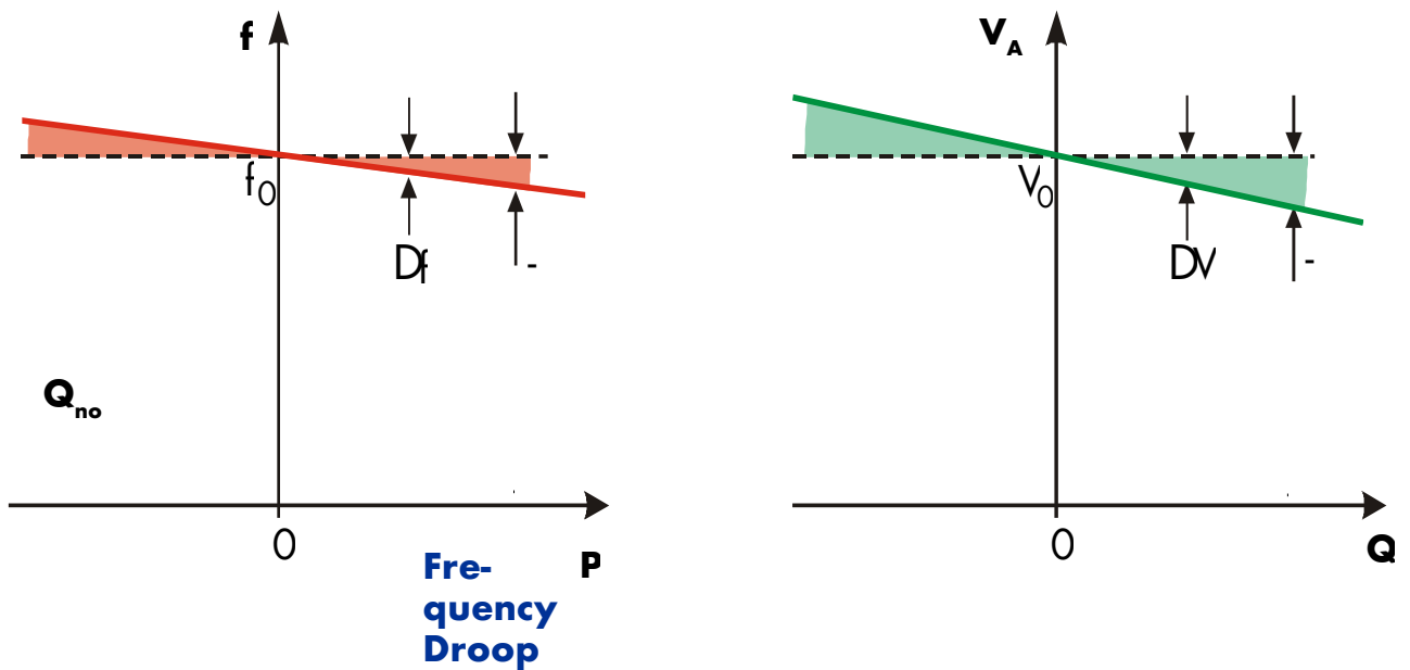
Figure 8.5: Self-sync - droop
