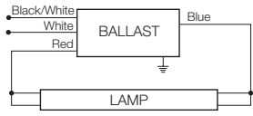
QUICKTRONIC 1x32
