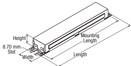
QUICKTRONIC 4x32
