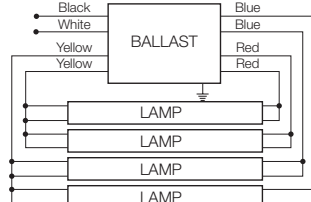
QUICKTRONIC 2x32
