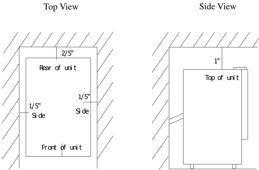
INSTALLATION CLEARANCES
