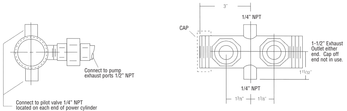
Figure 3 - Exhaust Manifold TB-1126 (optional)
