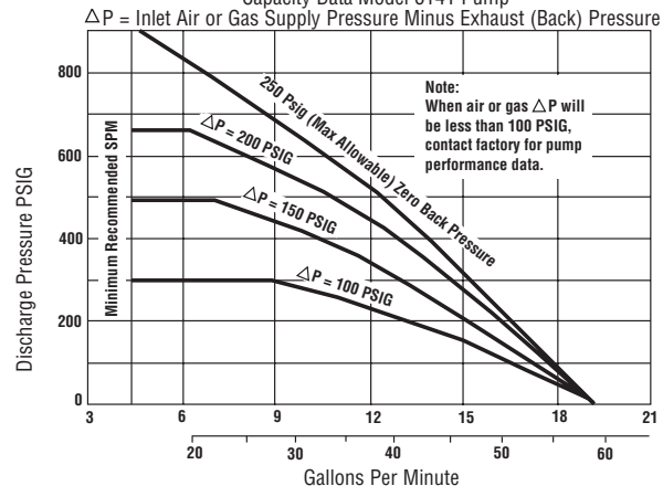
Capacity Data Model 6141 Pump
