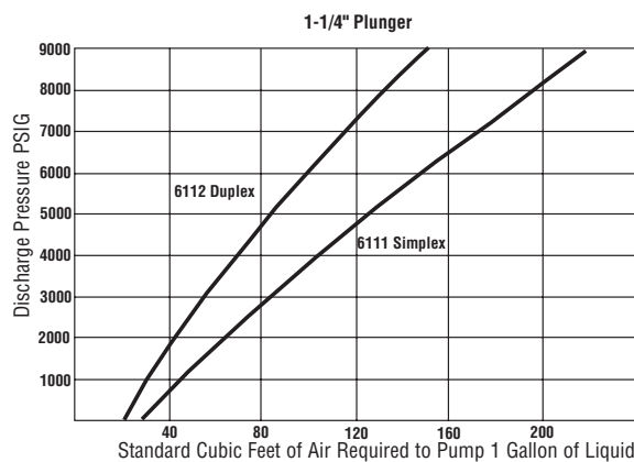
Air Consumption Models 6111 & 6112 (Zero Back Pressure)
