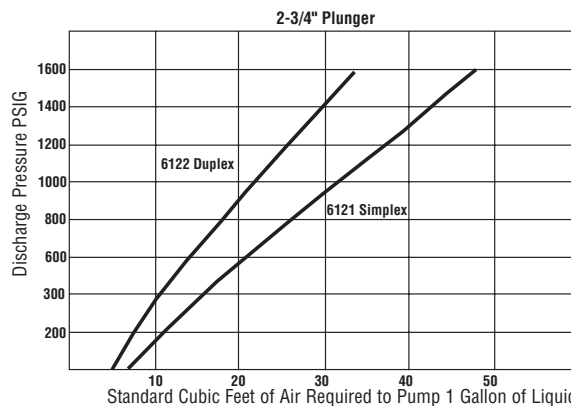
Air Consumption Models 6121 & 6122 (Zero Back Pressure)
