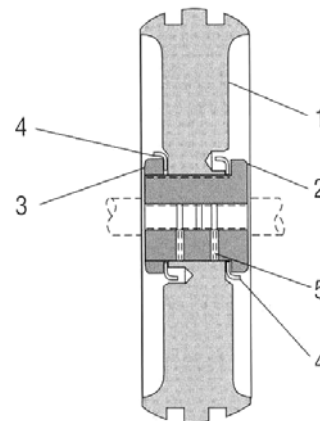
TB-813 Power Piston (Item 22, Page 4)
