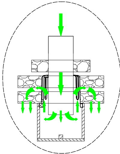
Defoaming device
