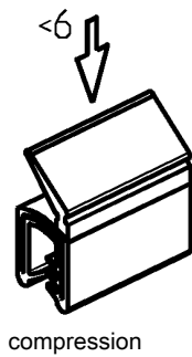
Sponge-rubber (EPDM) black (gasket EPDM 60° ± 5 Shore A)
