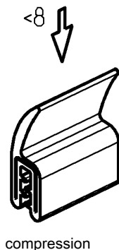
Gasket EPDM 60° ± 5 Shore A black
