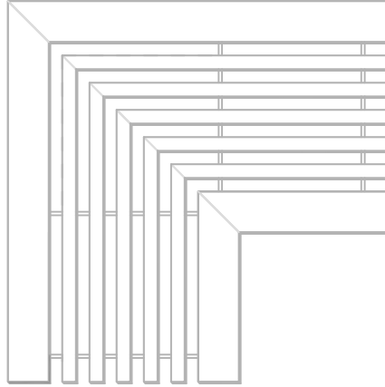
Plan of Bar Grille with frame
