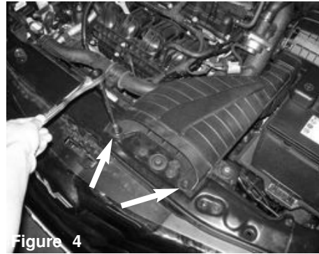
Figure 4 Use a 10mm socket/ratchet and remove the two M6 bolts attached to the factory air box inlet duct.
