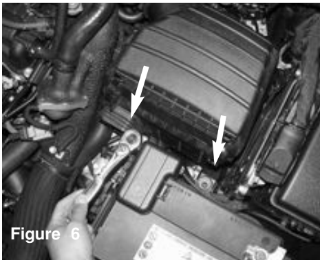
Figure 6 Use a 10mm socket/ratchet and remove the two M6 bolts in front of the air box assembly
