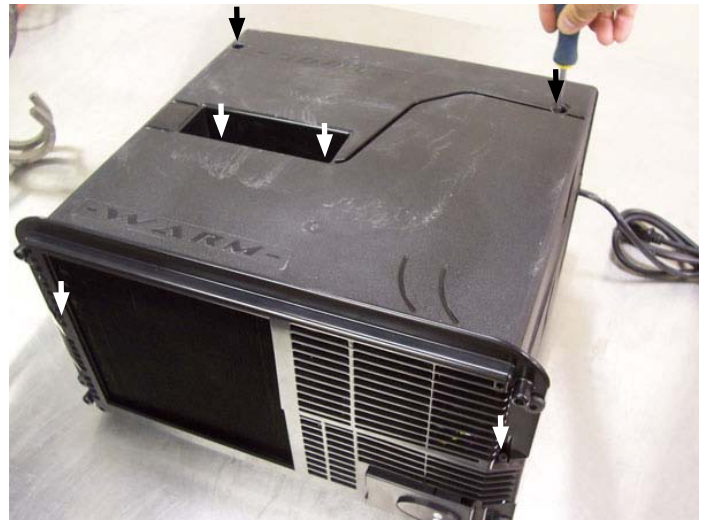
⑧ Screw in all 6 screws.
