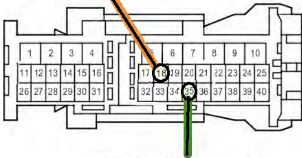
Picture 15: Pin side view
