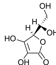
2. Ascorbic acid
