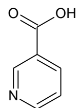
1. Nicotinic acid
