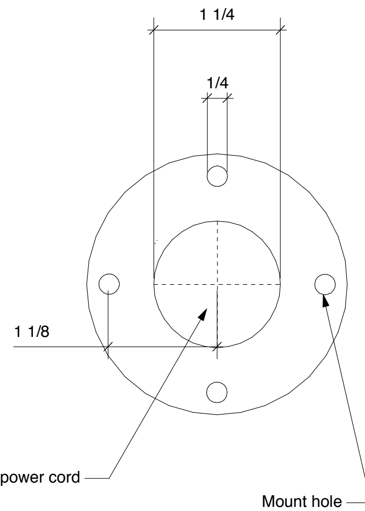
5 Mount Hole Detail
