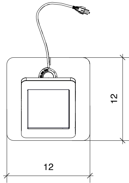
1 Top View
