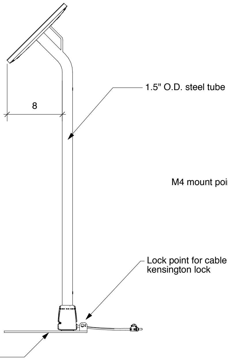
3 Right View
