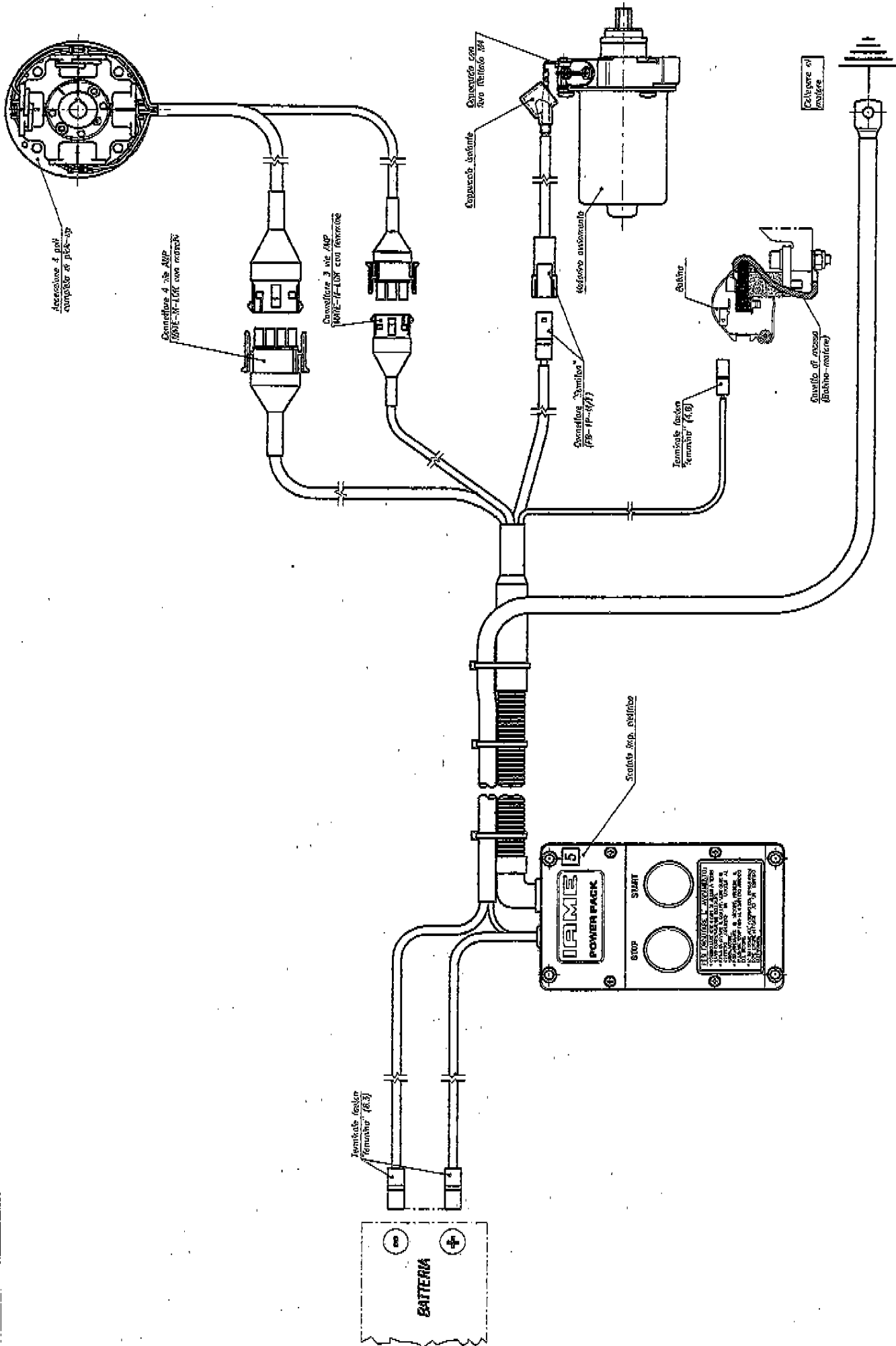
"DIGITAL 4 POLES" IGNITION WIRING DIAGRAM
