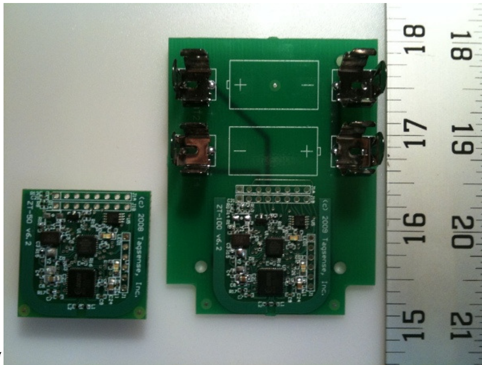
ZT-50 and ZT-100 Side by Side Comparison
