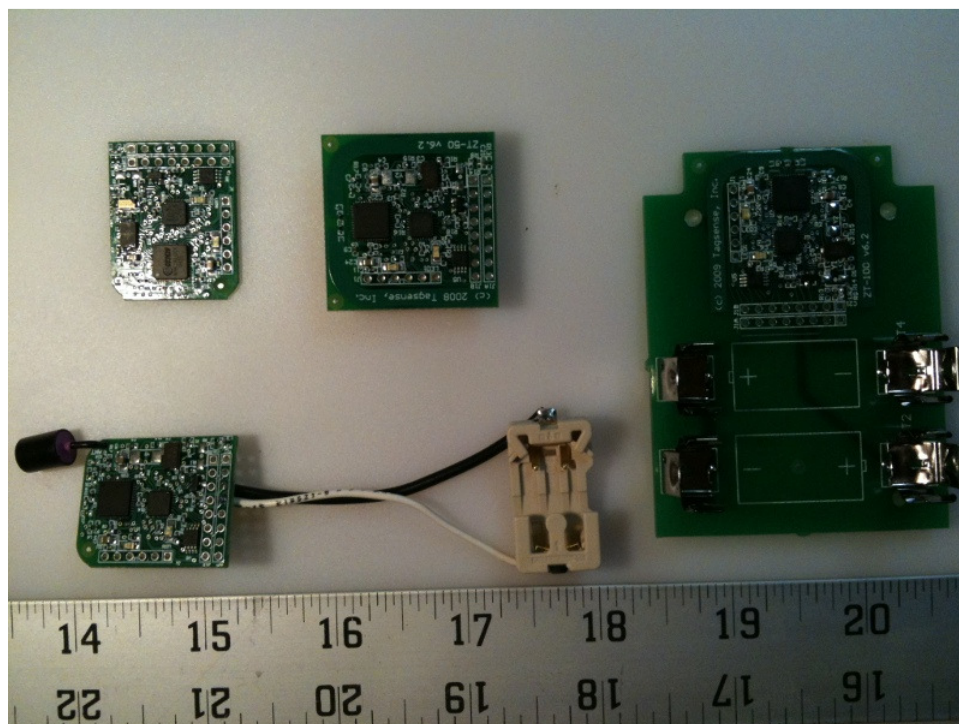
Starting from top left: ZT-50 Mini (standard), ZT-50, ZT-100, ZT-50 Mini with Battery holder and Antenna
