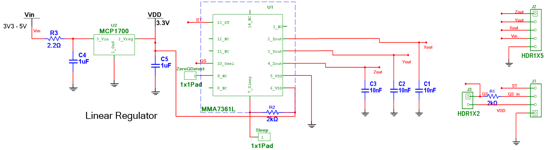
Modern Device MMA7361 3-Axis Accelerometer Board
