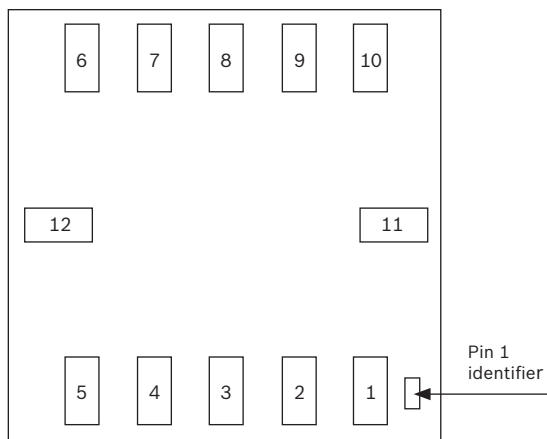
Pin configuration for SPI interface (bottom view)
